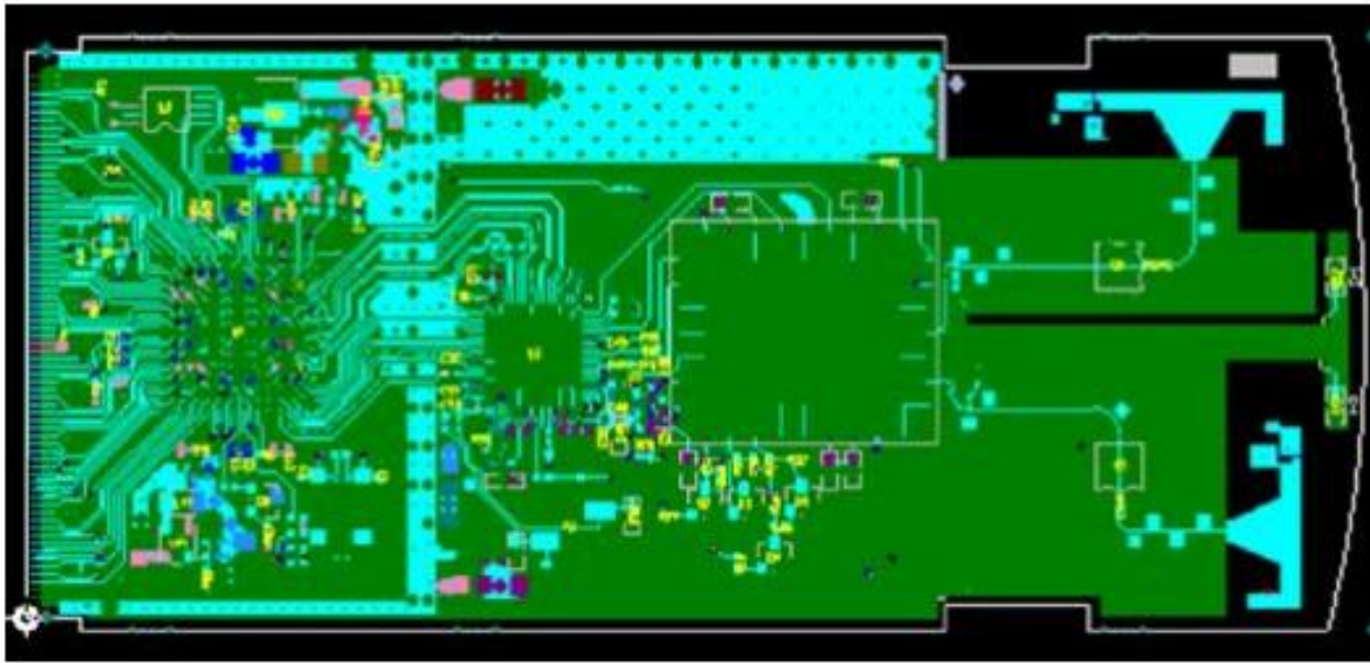
PCMCIA WIRELESS LAN CARD 4 layers
